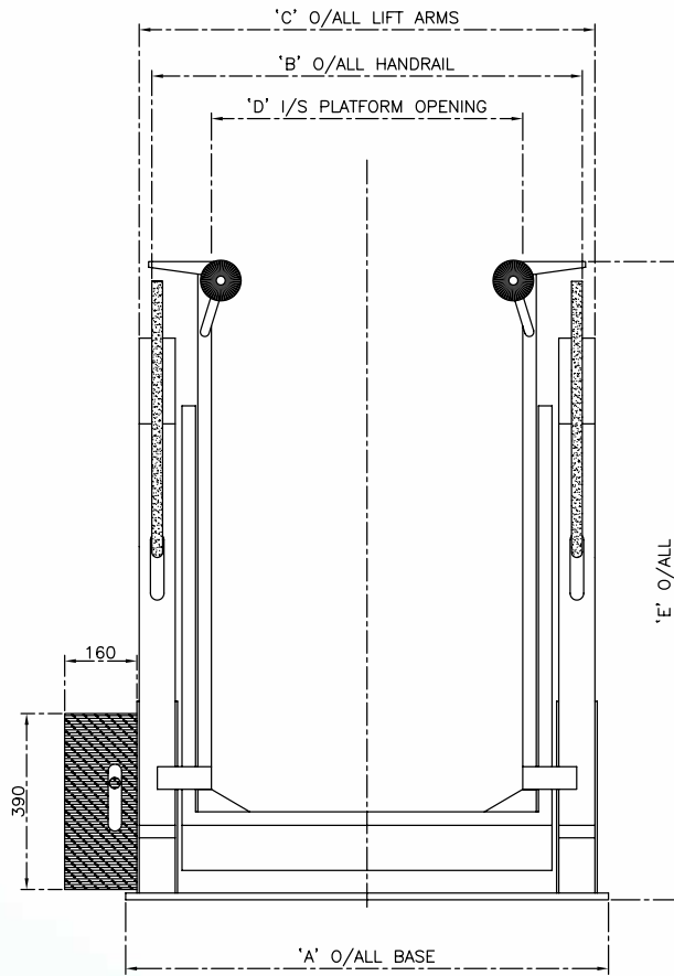
P.L.S. EASY ACCESS INBOARD LIFT
